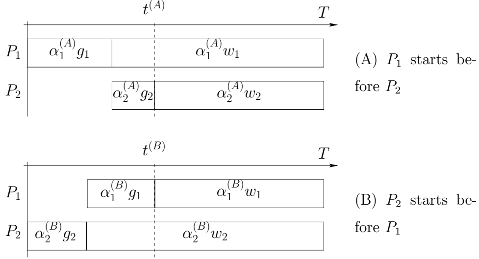
Fig. 4. Comparison of the two possible orderings.
