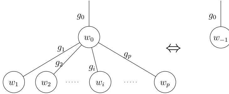
Fig. 5. Replacing a single-level tree by an equivalent node.
