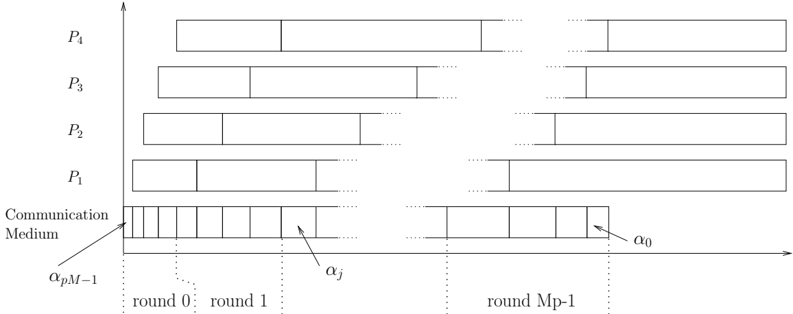
Fig. 6. Pattern of a solution for dispatching the load of a divisible job, using a bus network ( g_i = g ), in multiple rounds, for 4 workers. All 4 workers complete execution at the same time. Chunk sizes increase during each of the first M - 1 rounds and decrease during the last round.
