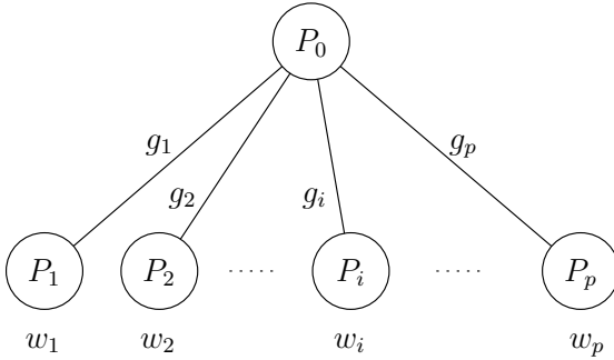
Fig. 1. Heterogeneous star graph, with the linear cost model. Fig. 2. Heterogeneous tree graph.
