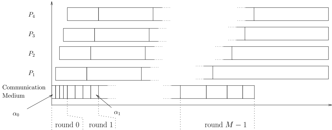
Fig. 7. Pattern of a solution for dispatching the load of a divisible job, using a bus network ( g_i = g ), in multiple uniform rounds, for 4 workers. All workers complete execution at the same time. Chunk sizes are fixed within the first M - 1 rounds but increase from round to round. Chunk sizes decrease during the last round.
