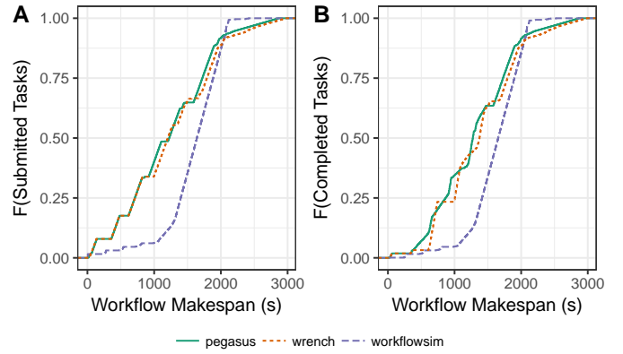
Fig. 4: Empirical cumulative distribution function of task submission times (left) and task completion times (right) for sample real-world (“pegasus”) and simulated (“wrench” and “workflowsim”) executions of Montage-2.0 on AWS-m5.xlarge.
