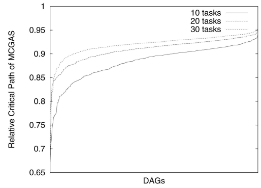
Fig. 4. Relative critical path length of MCGAS ( \mu = 0.66 and b = 87 ) compared to HCPA, for applications with 10, 20, and 30 tasks.
