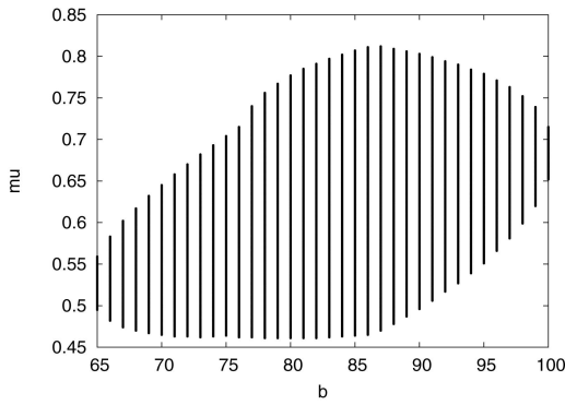
Fig. 3. Domain of b and \mu values for which MCGAS's performance ratio is lower than 10, for our particular platform configuration.
