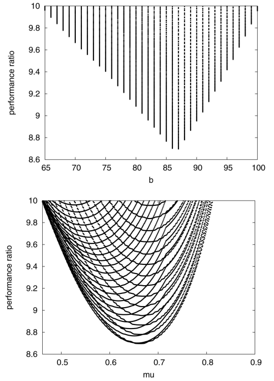
Fig. 2. 2D projections of all (\mu, b, 1/\beta) triplets with performance ratio 1/\beta lower than 10.
