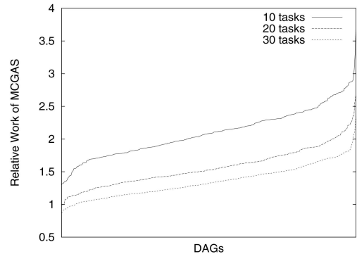
Fig. 5. Relative total work of MCGAS ( \mu = 0.66 and b = 87 ) compared to HCPA, for applications with 10, 20, and 30 tasks.
