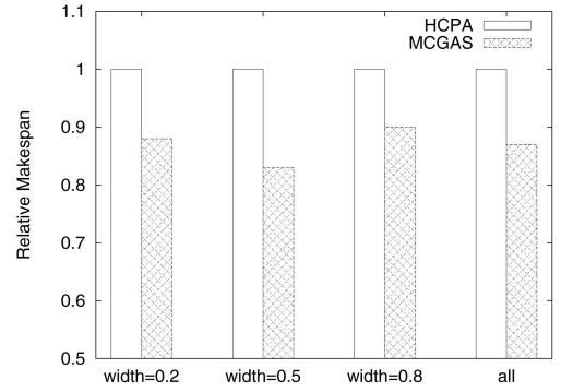
Fig. 7. MCGAS versus HCPA using \mu = 0.81 , b = 87 .
