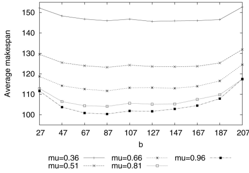
Fig. 6. Evolution of the average makespan obtained with the MCGAS algorithm as b varies. Each curve is for a different \mu value.
