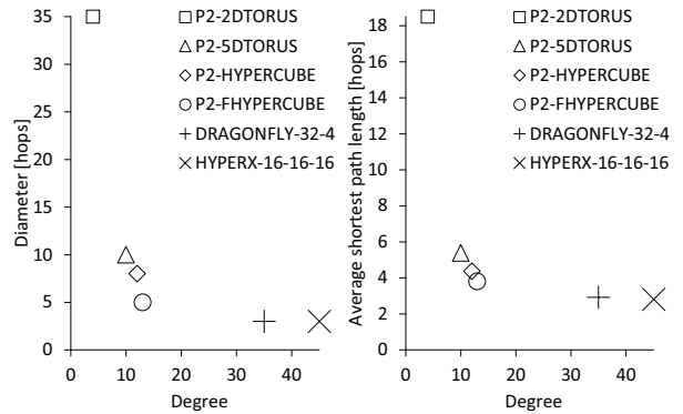
Fig. 6. Diameter (left) and average shortest path length (right) vs. degree for 4,096-switch direct networks including DRAGONFLY and HYPERX.
