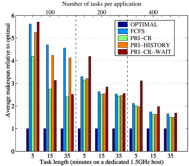
Figure 3: Performance of resource prioritization heuristics on the SDSC grid.
