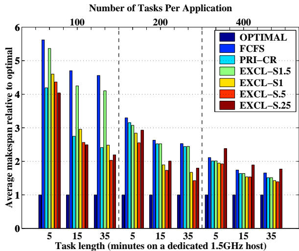
Figure 5: Performance of heuristics using thresholds on SDSC grid
