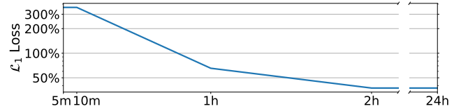
Figure 1: Loss value vs. time when using all ground-truth data for the Epigenomics workflow.
