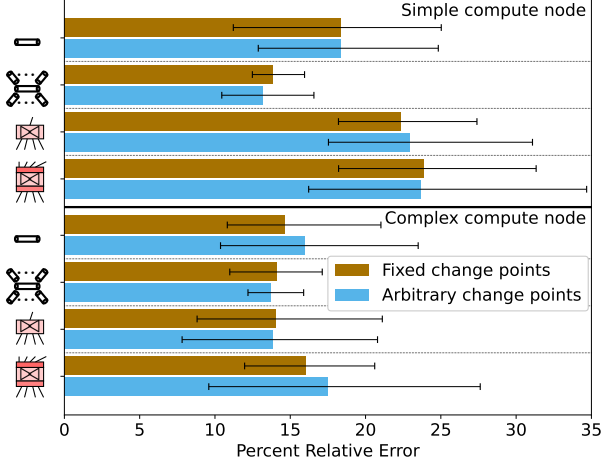
Figure 5: Percent relative error between simulated and ground-truth data transfer rates (bars show average values over all benchmarks; error bars show min and max values). The top, resp. bottom, half of the figure is for simulating a simple, resp. complex, compute node. Each pair of bars is for one of the four options for simulating the network topology (depicted as simplified network diagrams on the vertical axis). Each bar in a pair is for a different option for simulating the adaptive MPI protocol, with either fixed or arbitrary change points.
